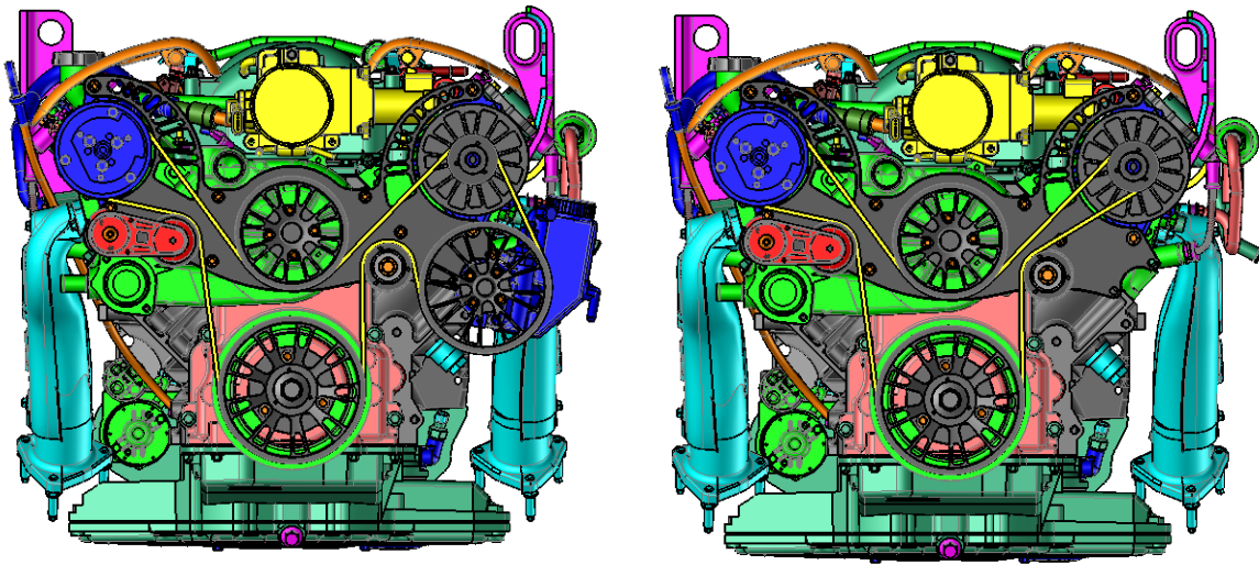
Belt Install with alternator pulley
